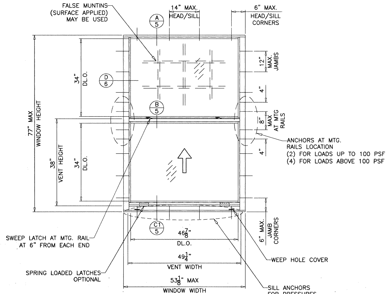
TYPICAL ELEVATION (HI-RISE FRAME SILL) (TESTED UNIT)
